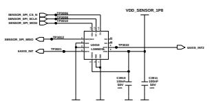
ACC&GYRO SENSOR
