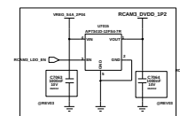
RCAM3 LDO
