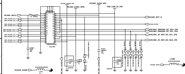
RCAM1_24M CAMERA(34PIN)_IMX576
