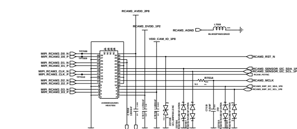
RCAM3_SUPER WIDE 8M CAMERA(30pin)_S5K4HA
