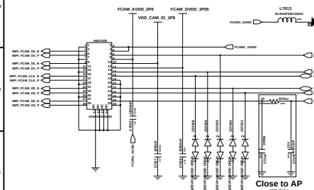
FRONT_CAMERA (24M)
