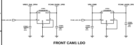
FRONT CAM1 LDO
