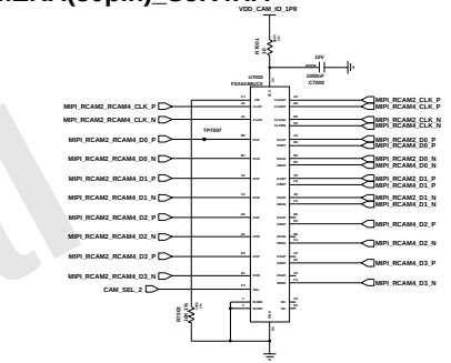
MIPI SWITCH (RCAM2,RCAM4)
