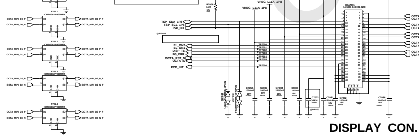
OCTA FILTER
