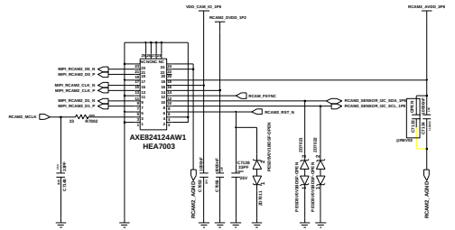
RCAM2_5M CAMERA(24PIN)_S5K5E9
